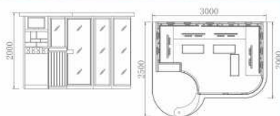
D6-K8 Size: 3000×2500×2000mm
