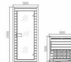
KY002 Size: 900×900×1980mm
