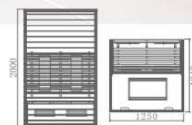
08-K72 Size: 1250×1240×2000mm
